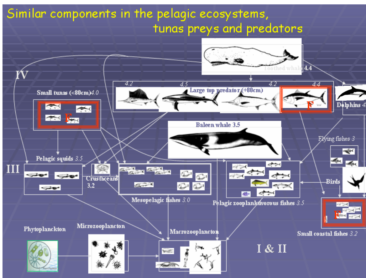
Figure 2. Schematic representation of the pelagic food web (by Alain Fonteneau, IRD, France)
