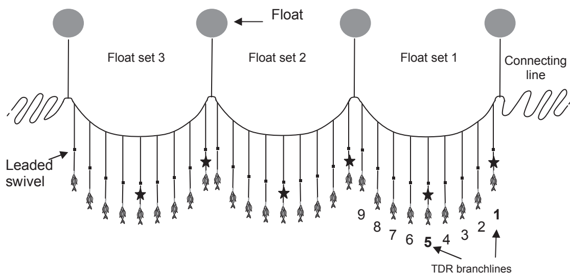
Figure 2. Gear configuration and position of time-depth recorder (TDR) branch lines used in the experiment. As indicated, each treatment of mainline tension comprised three float sets and each float set comprised two TDR positions.
