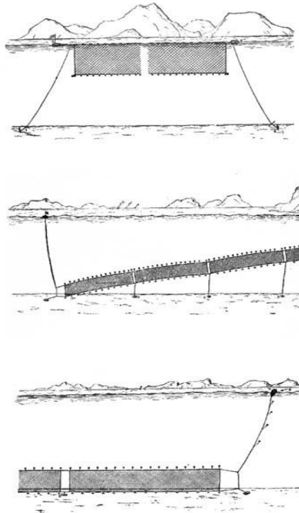
Figure 14. three variations on the placement and design of gillnet gear (source: NOAA)
