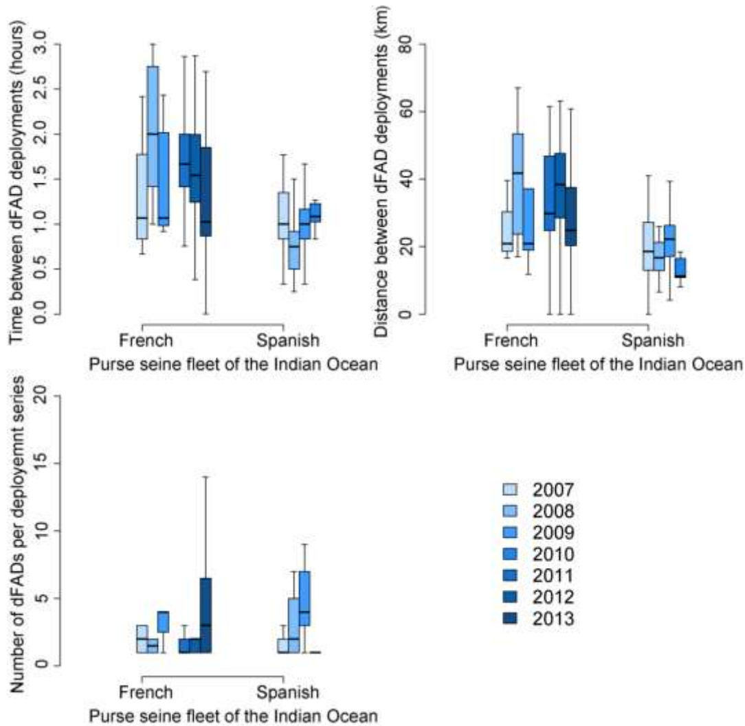
Figure 5: yearly time, distance and number of dFAD deployments per series for the French and Spanish fleets
