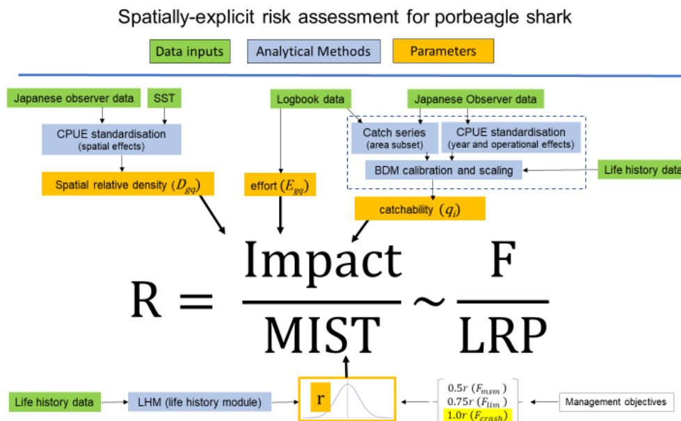
Figure 17. Conceptual representation of data inputs, analytical methods and key parameters used in spatially-explicit risk assessment of the Southern Hemisphere porbeagle shark. BDM = Bayesian state-space biomass dynamics model. The dashed outline box represents analytical methods applied to a region subset of the available data.
