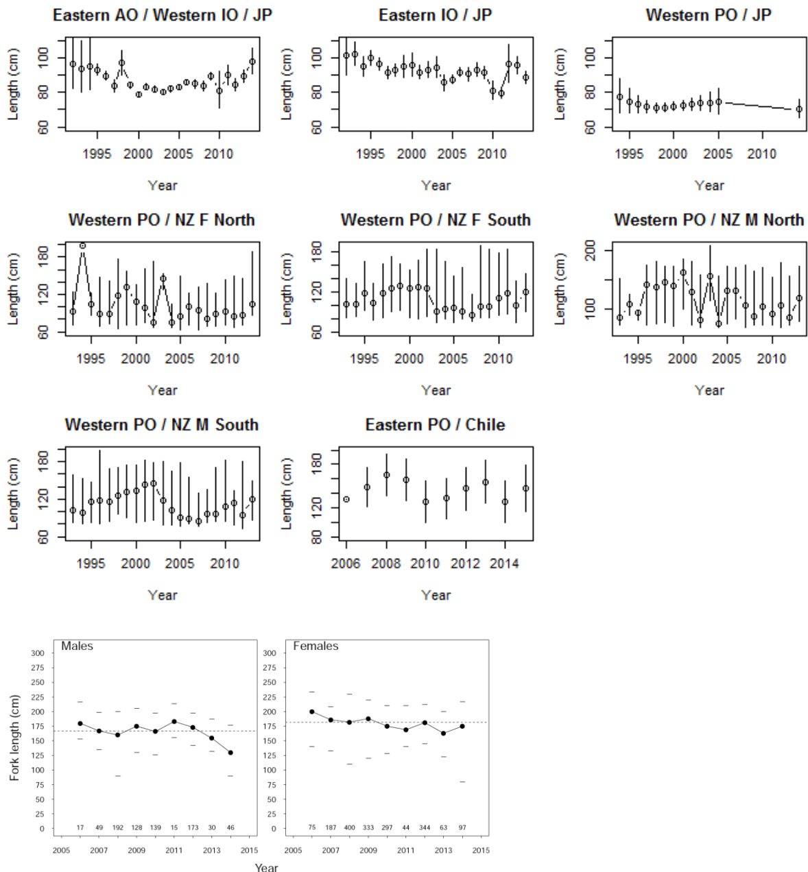
Figure 15: Standardized predictions (Japan (JP) and Chile) and annual measurements (New Zealand (NZ) and Argentina) of lengths in the catch, by region and contributing country. Sources: (Cortés et al. 2017, Francis & Large 2017, Hoyle et al. 2017b, Hoyle et al. 2017a).
