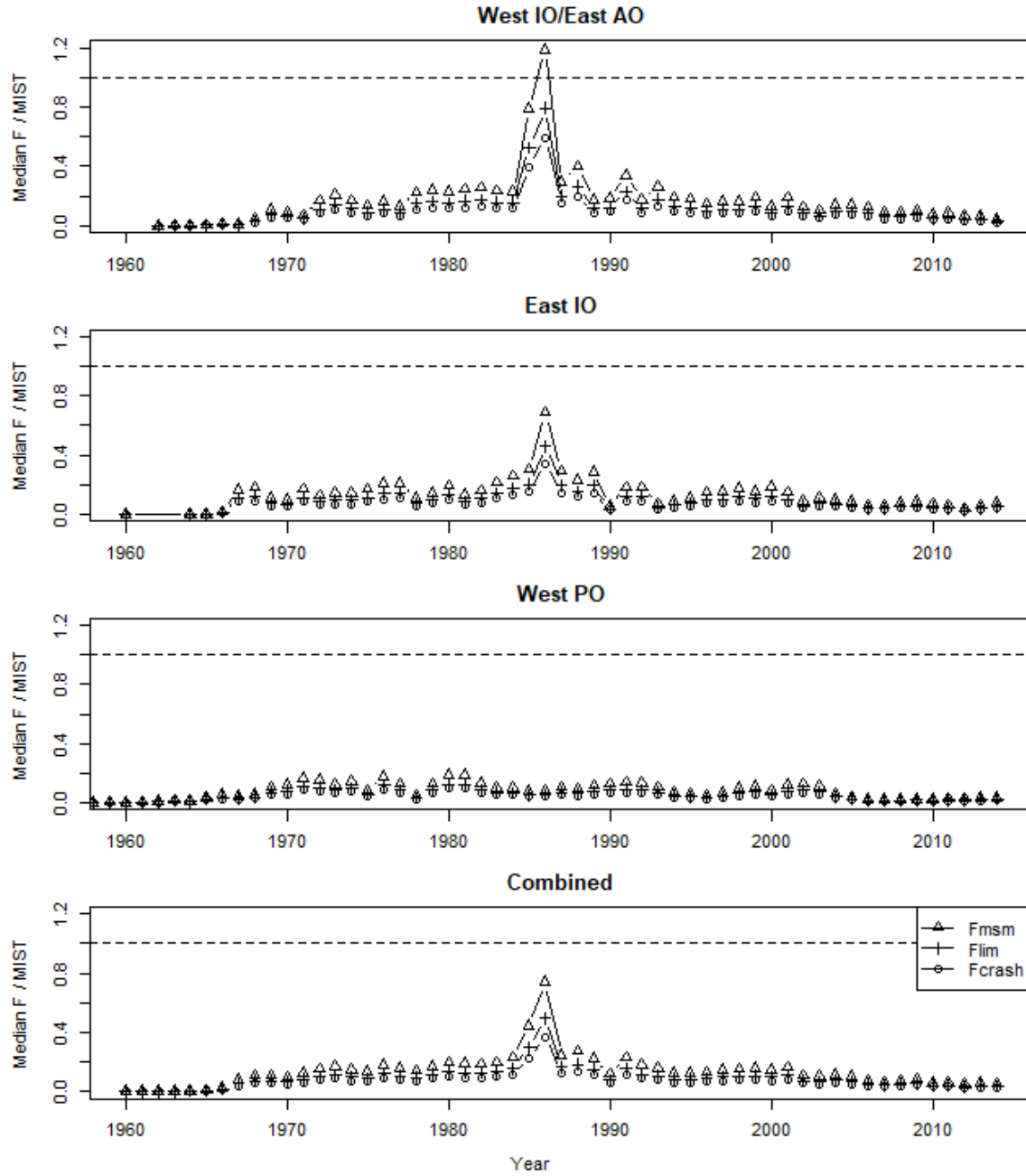
Figure ADD2: F-ratio plots showing the median values of F / MIST by year, for the three versions of the MIST ( F_{msm} , F_{im} , and F_{crash} ) for each of the three regions and for the three regions combined (the assessment area). Note that the F-ratio is almost always below 1, indicated by the horizontal dotted line.
