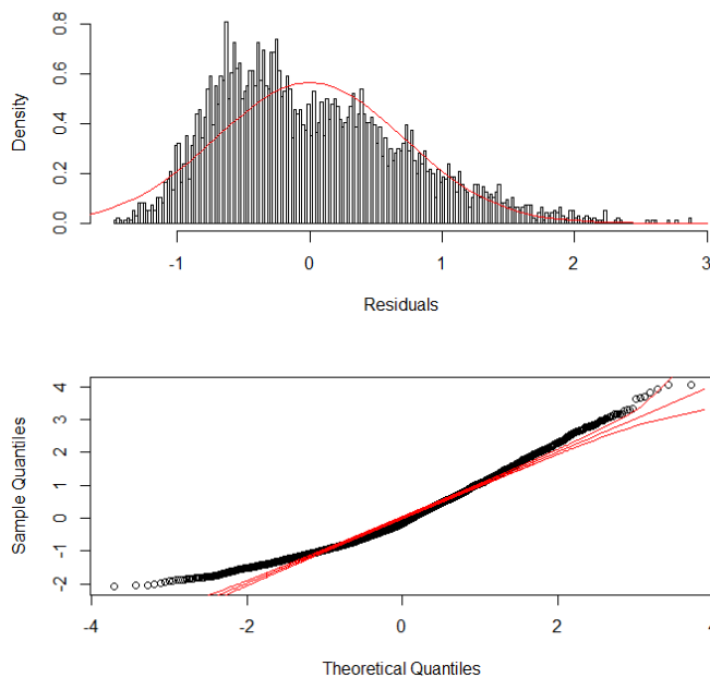
Figure 7: Residual distribution plots for the lognormal positive observer data analysis for catch prediction.
