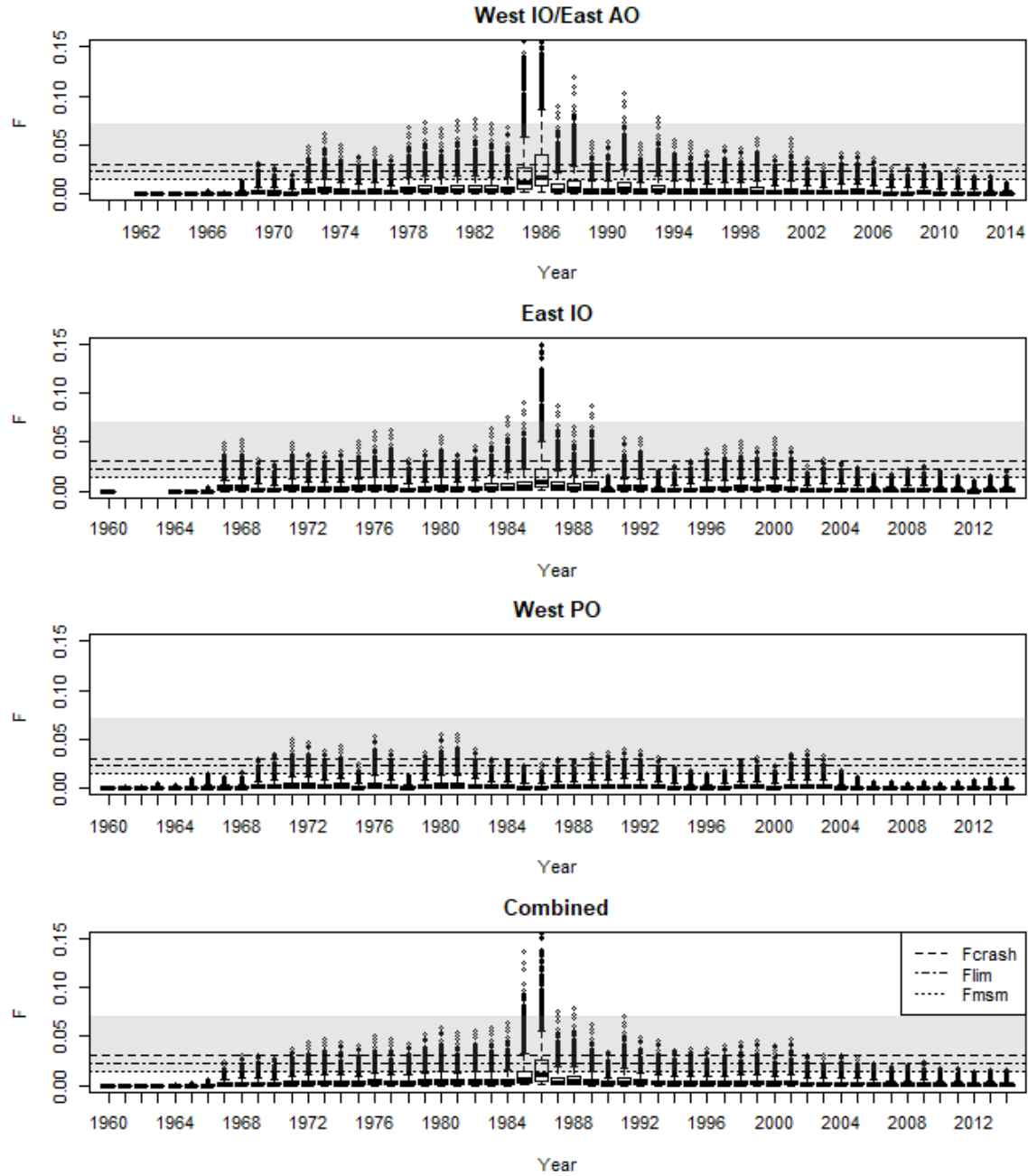
Figure ADD1: Estimated fishing mortalities by year and region. The horizontal dotted lines indicate the median MIST values ( F_{crash} , F_{lim} , and F_{msm} ), but note that the MIST varies among realisations of the model, with the grey band showing the 90% distribution for F_{crash} . The boxes show the interquartile range of the F estimates, with a line at the median of each. The whiskers extend up to 1.5x the interquartile range. Dots mark points beyond the whiskers.
