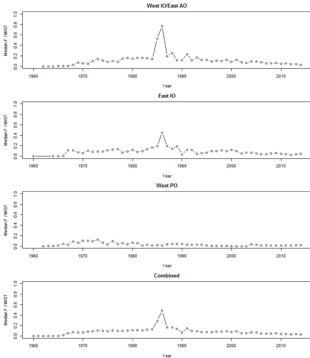
Figure 22: F -ratio plots showing the median values of F / MIST by year, for three regions, and for the three regions combined (the assessment area). Note that the F -ratio is always below 1, which is the upper bound of the y axis.
