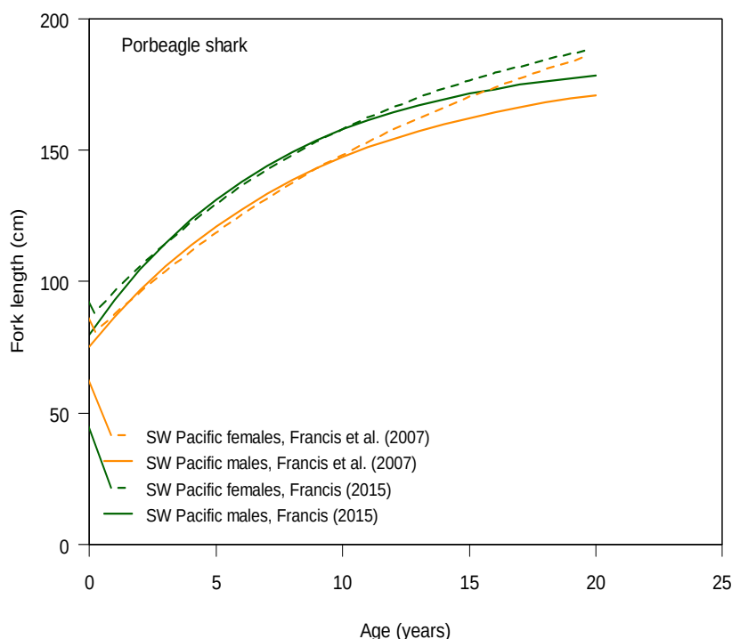
Figure 2. Growth curves for porbeagle shark (reproduced from Clarke et al. 2015).
