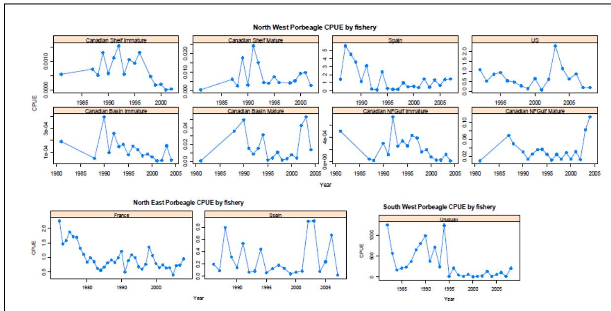
Figure 3. Catch per unit effort series for the northwest Atlantic (upper figures), northeast Atlantic (lower left figures) and southwest Atlantic (lower right figures) stocks (ICCAT 2010).
