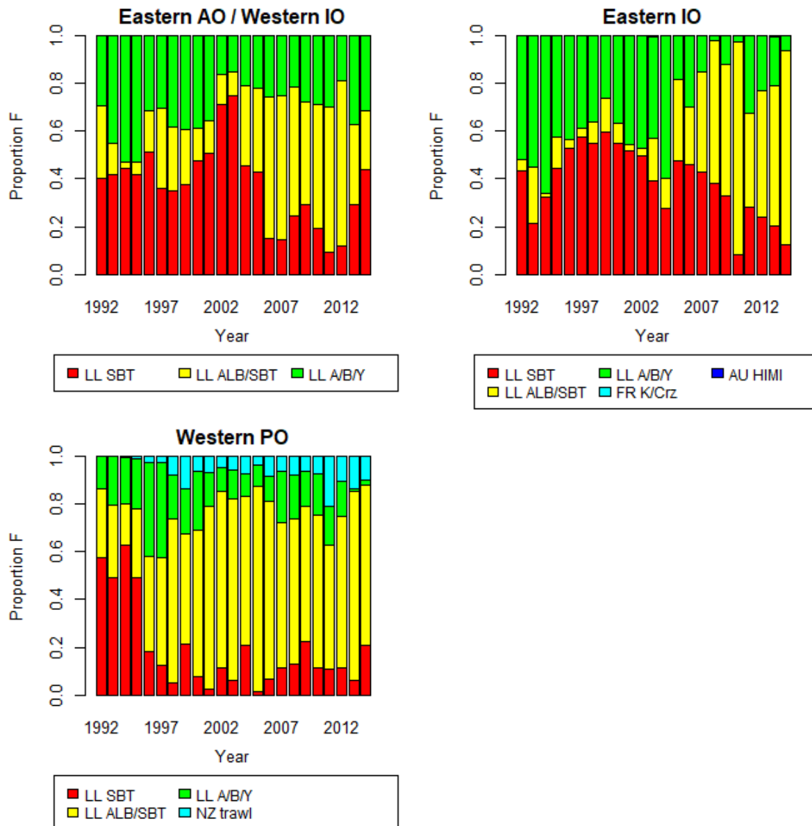
Figure 24: Proportional contributions by year and region to fishing mortality, for the fisheries operating in each region. The pelagic longline effort is broken into three fishing strategies based on cluster analysis (see Hoyle et al. 2017). Note that the French (Kerguelen and Crozet Islands) and Australian (Heard Island and McDonald Islands) sub-Antarctic fisheries' contributions to F are too small to be visible on the plots.
