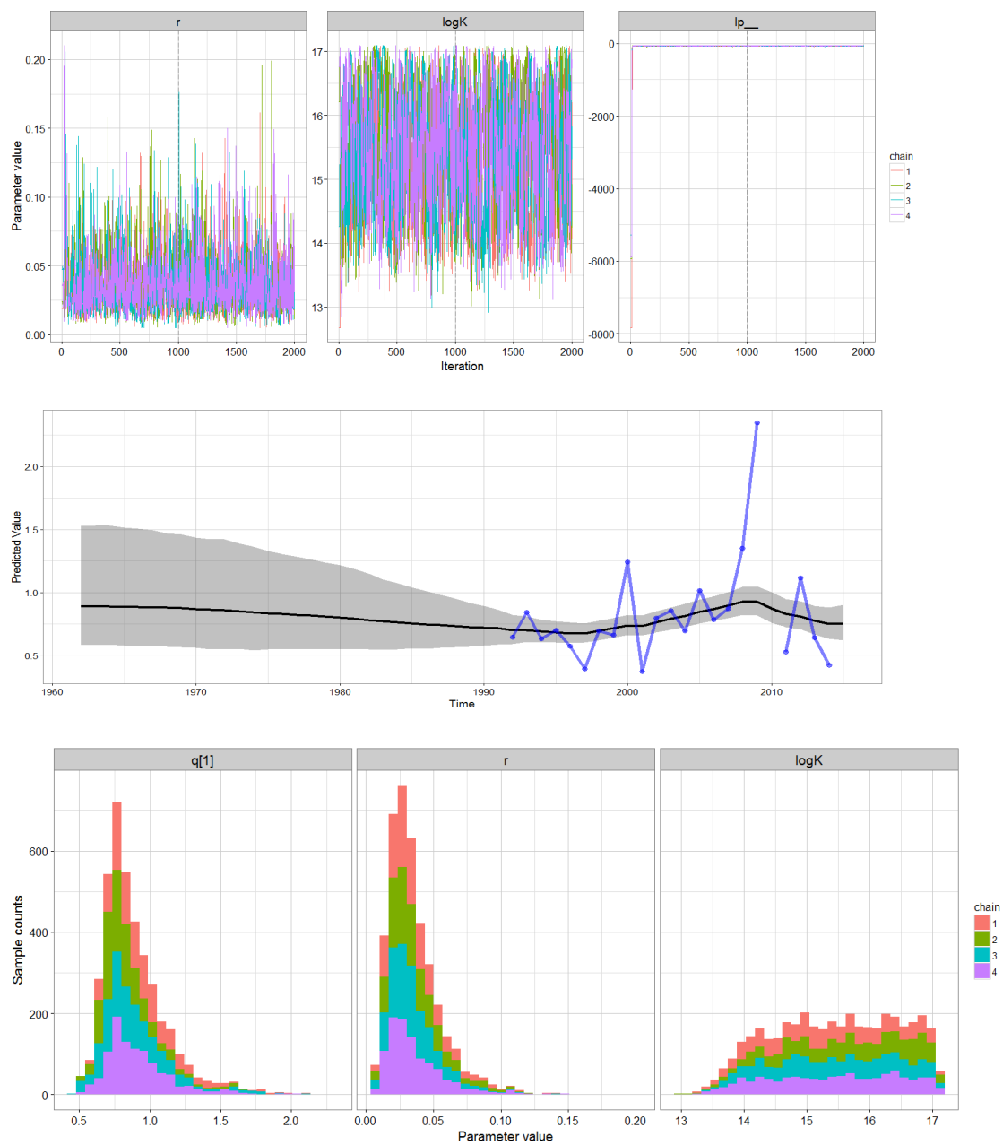
Figure 20. Top: Trace outputs from the MCMC model fit showing estimates of r and \log(K) alongside the log-posterior ( lp\_ ). Middle: Derived fit to the CPUE index. Bottom: Posterior distributions of q , r and \log(K) .
