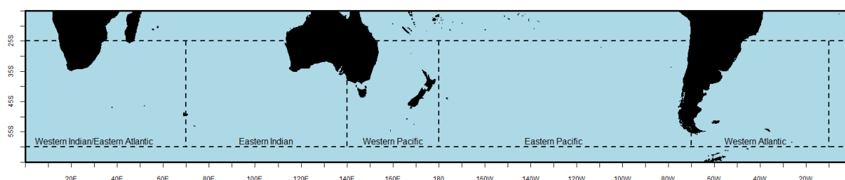
Figure 6: Spatial subdivision of the Southern Hemisphere porbeagle population into five regions.
