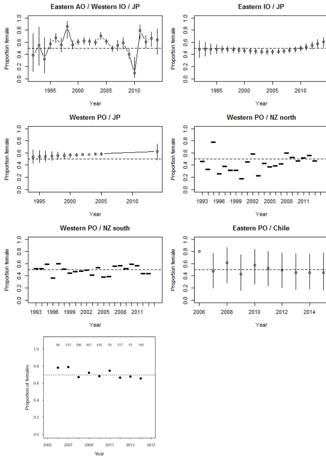
Figure 16: Standardized predictions (Japan (JP) and Chile) and annual measurements (New Zealand (NZ) and Argentina) of proportion female in the catch, by region and contributing country. Sources: (Cortés et al. 2017, Francis & Large 2017, Hoyle et al. 2017b, Hoyle et al. 2017a).
