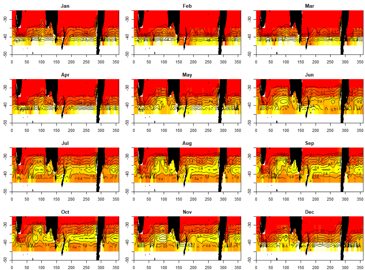
Figure 11: Predicted population relative distribution by month from the abundance prediction model. For each month, the area with highest density is assigned relative density of 1. Yellow indicates higher density, and red lower density. White indicates no information.
