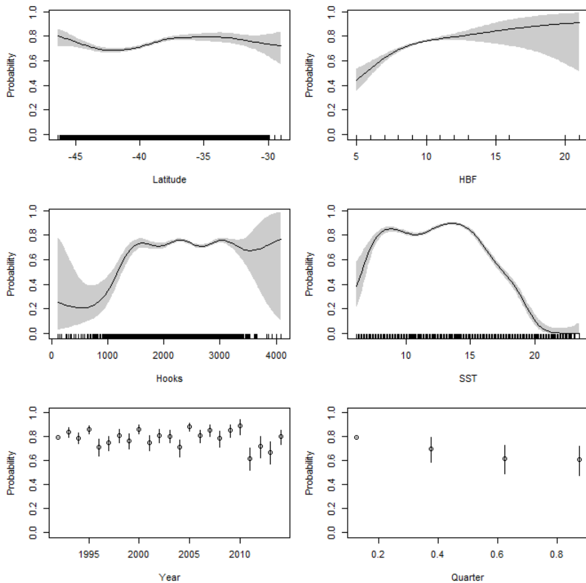
Figure 8: Probability of nonzero catch predicted for pelagic longline effort, for values of each covariate with other values held fixed. Fixed values were latitude 40 °S, HBF 11, SST 12 °C, Year 1992, and Quarter 0.125 (first quarter).
