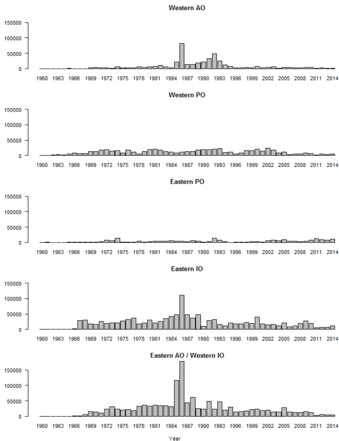
Figure 12: Total catch in number of porbeagle sharks per year by region.
