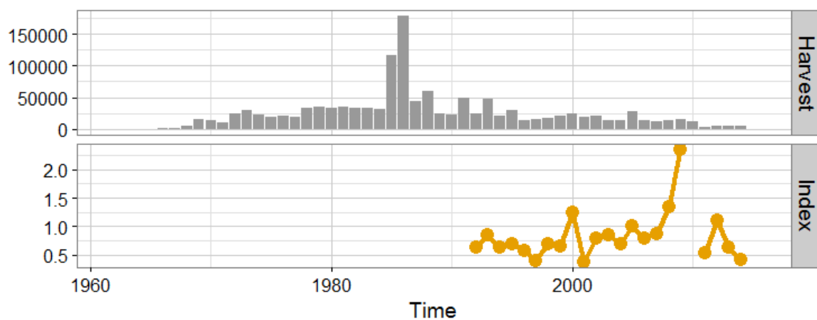
Figure 19. Catch and abundance data.
