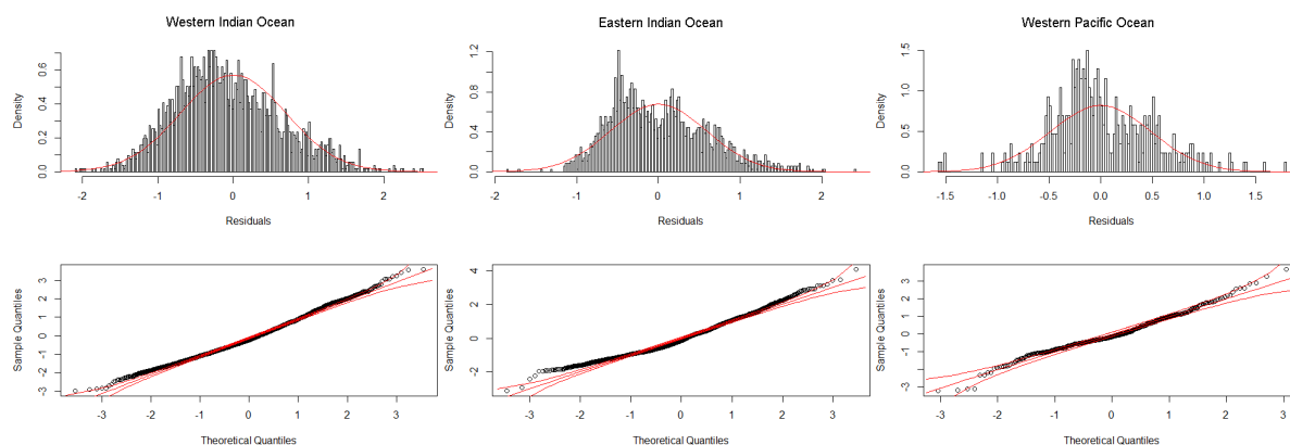
Figure 13: Residual distribution plots for lognormal positive observer data analyses for the Western and Eastern Indian Ocean, and the Western Pacific Ocean.
