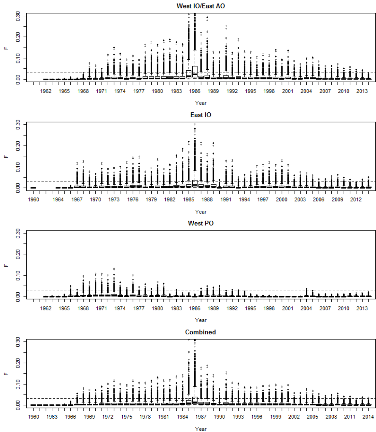
Figure 21. Estimated fishing mortalities by year and region. The horizontal dotted line indicates the median MIST value, but note that the MIST varies among realisations of the model, with the grey band showing the 90% distribution. The boxes show the interquartile range of the F estimates, with a line at the median of each. The whiskers extend up to 1.5 x the interquartile range. Dots mark points beyond the whiskers.
