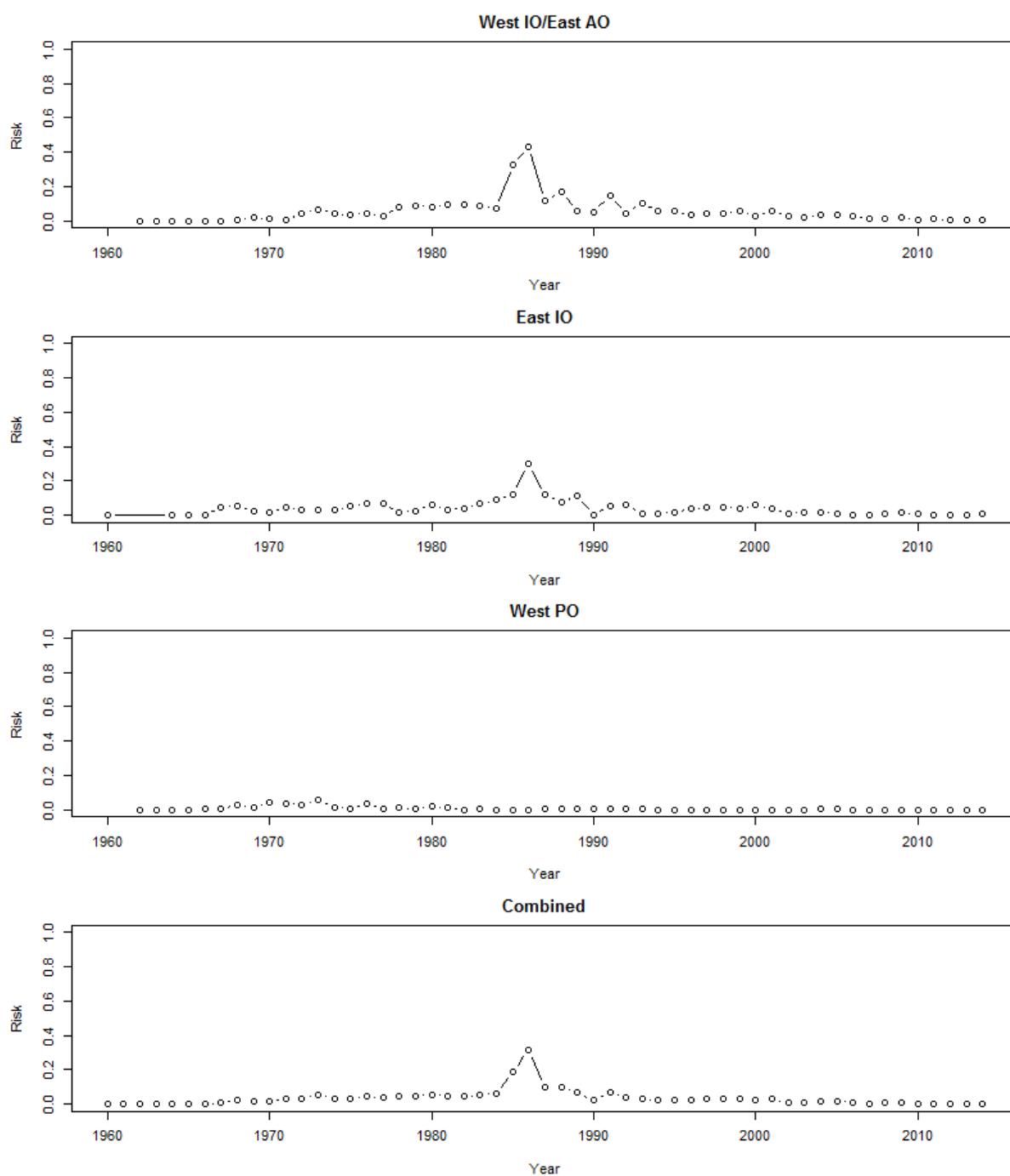
Figure 23: Risk plots showing the probability that F exceeds the MIST by year, for three regions, and for the three regions combined (the assessment area).
