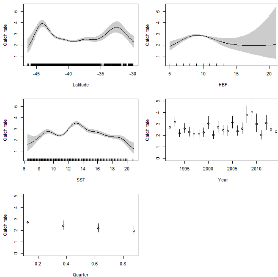
Figure 9: Predicted catch rate for nonzero pelagic longline effort, for values of each covariate with other values held fixed. Fixed values were latitude 40 °S, HBF 11, SST 12 °C, Year 1992, and Quarter 0.125 (first quarter).
