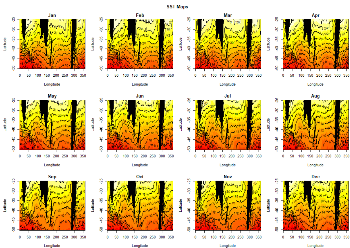
Figure 10: Sea surface temperature patterns by month from CARS data. Yellow represents higher SST, and red lower SST.
