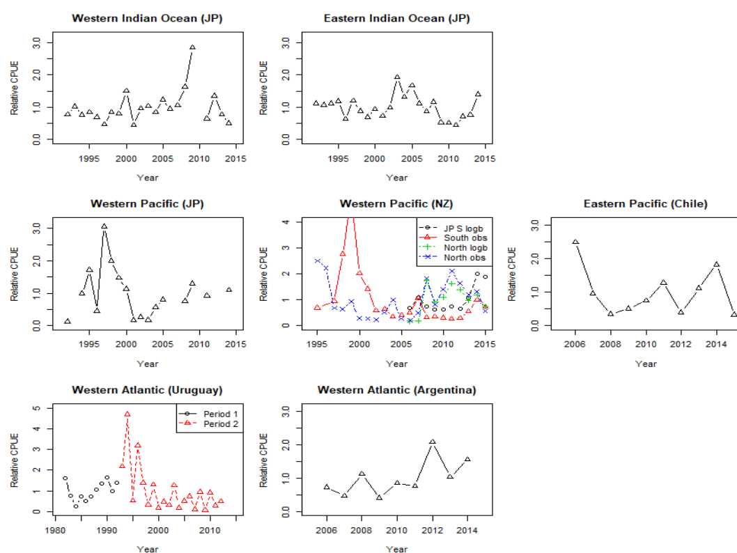
Figure 14: CPUE indices for each region and contributing country. Sources: (Cortés et al. 2017, Forselledo et al. 2017, Francis & Large 2017, Hoyle et al. 2017b, Hoyle et al. 2017a).
