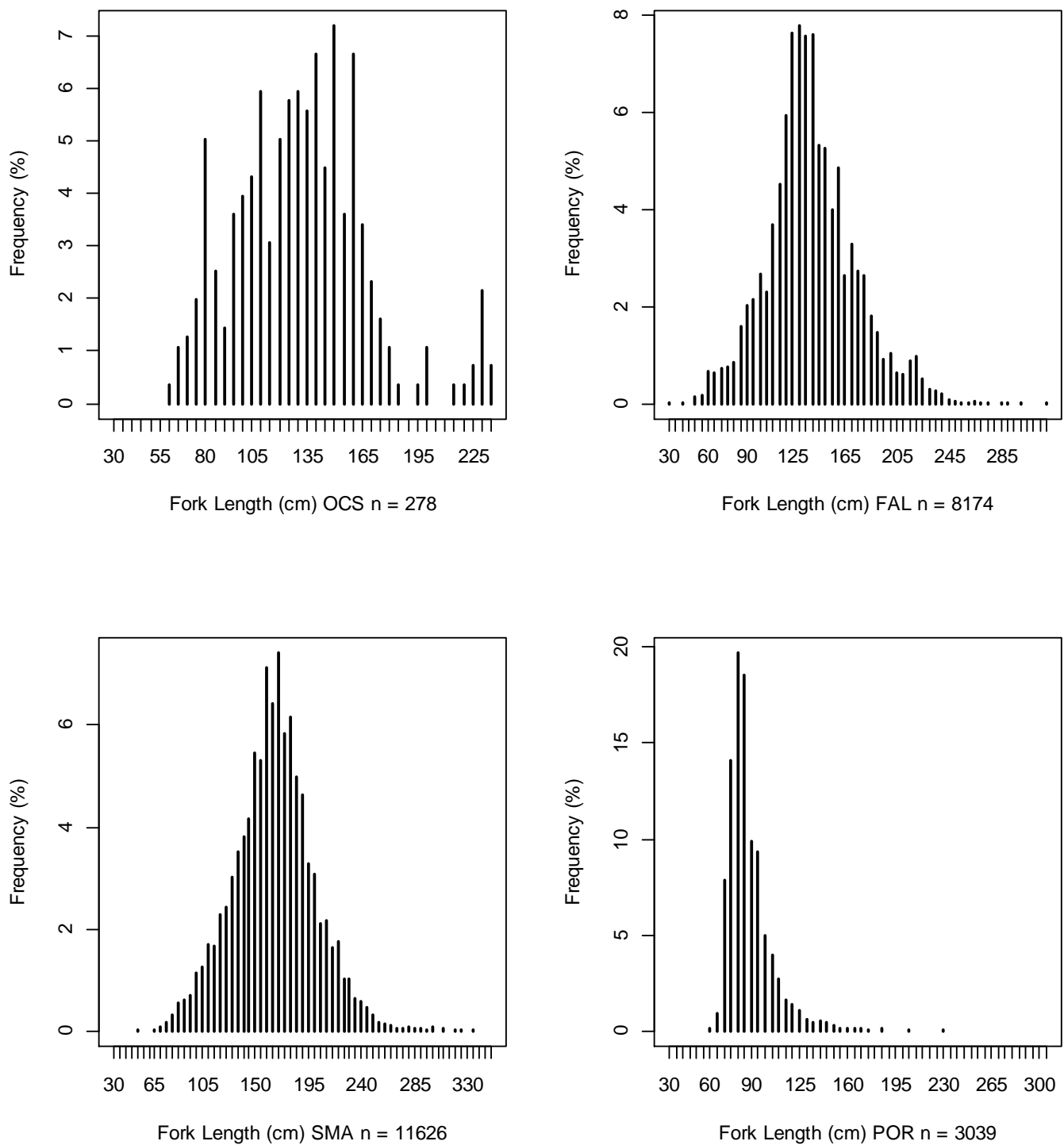
Fig. 13. Fork length frequency distributions (%) for oceanic whitetip shark (OCS), shortfin mako shark (SMA), porbeagle shark (POR) and silky shark (FAL) between 2005 and 2017.
